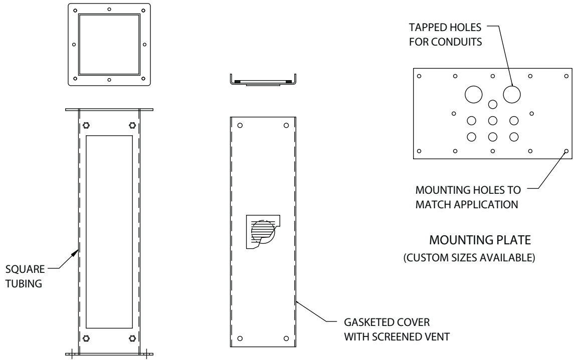
ALUMINUM PEDESTAL (CUSTOM SIZES AVAILABLE)
