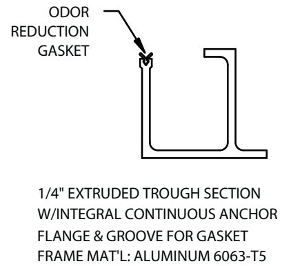
FRAME DETAIL
