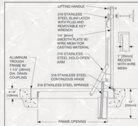
Model R-TPS
