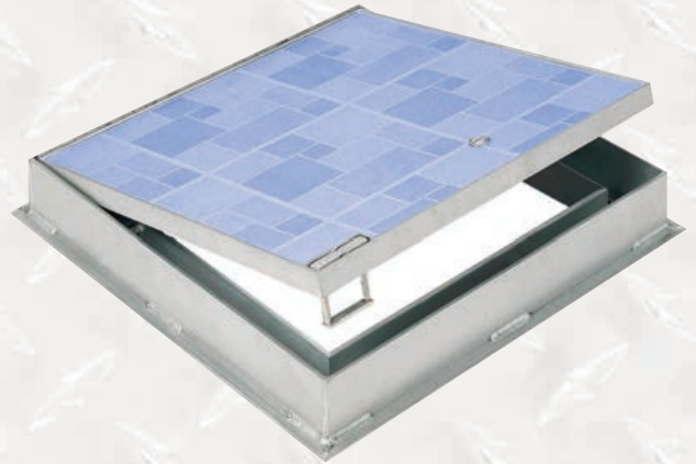
R-TPS Recessed Floor Door 1" [25mm] recess for concrete, stone or architectural tile
