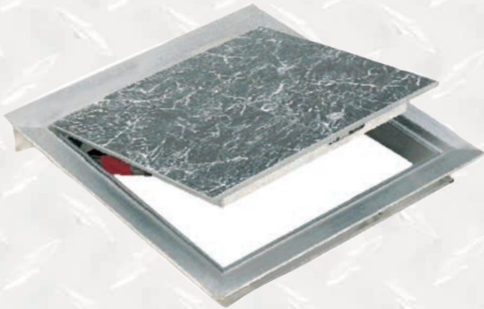
R-APS Recessed Floor Door 1/8" [3mm] recess for tile or carpet
