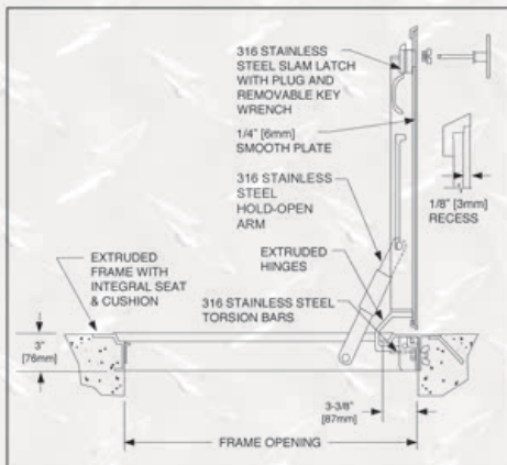
Model R-APS
