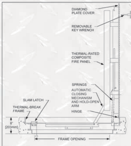
Model FD
