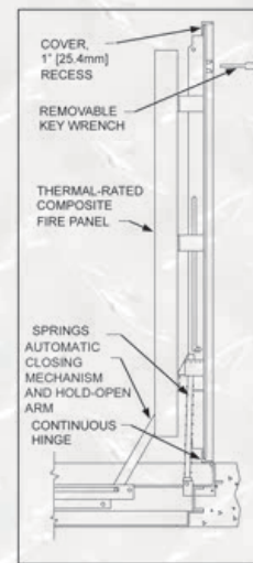
Model FD-P
