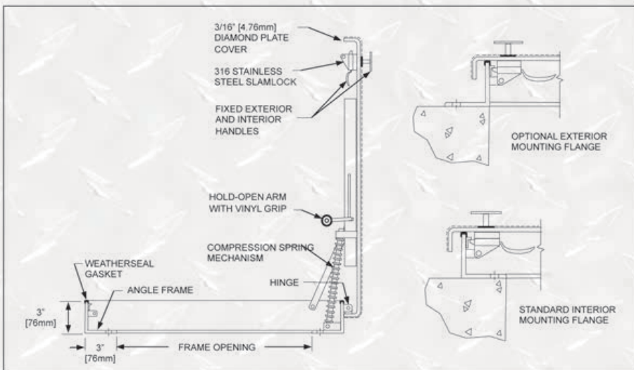
Model SRR
