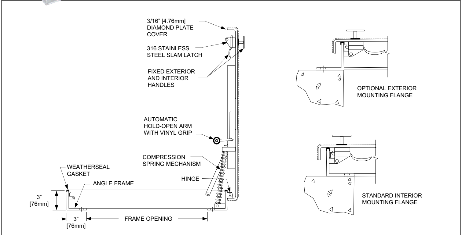
Model SRR-E with optional Exterior Mounting Flange, Padlock Staple and Lifting Handle
