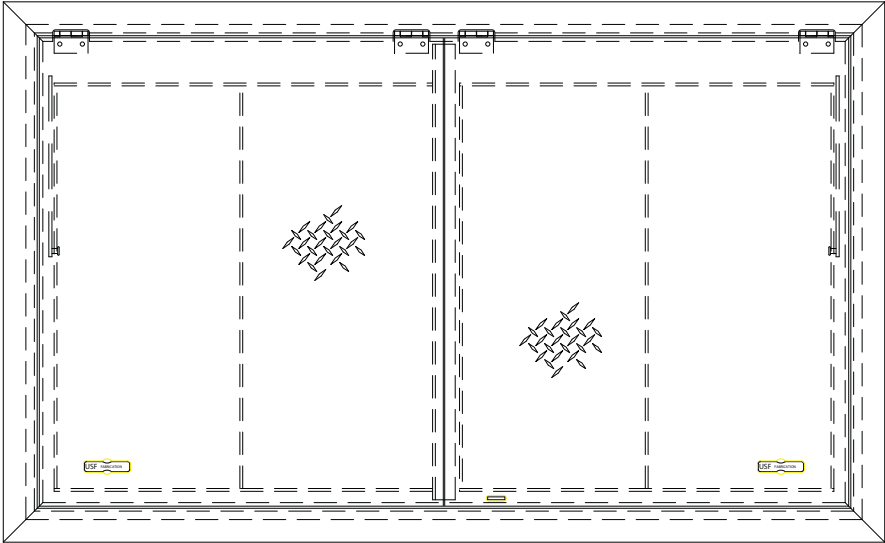
DOUBLE DOOR HINGED ON THE SAME SIDE
