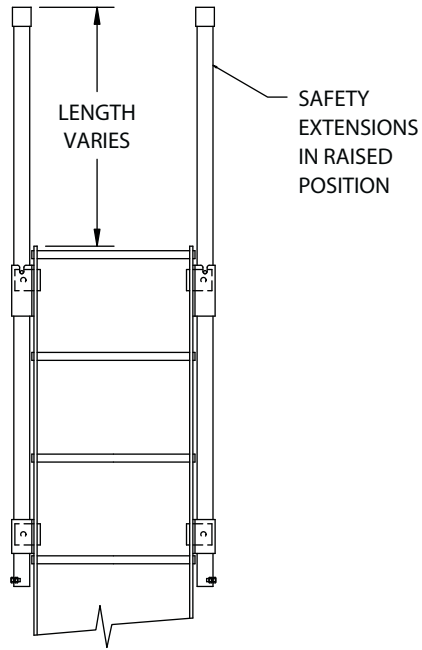
LADDER WITH SAFETY EXTENSIONS
